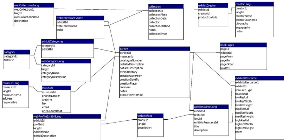
Figure 1 – Core database schema for integrated museum system
